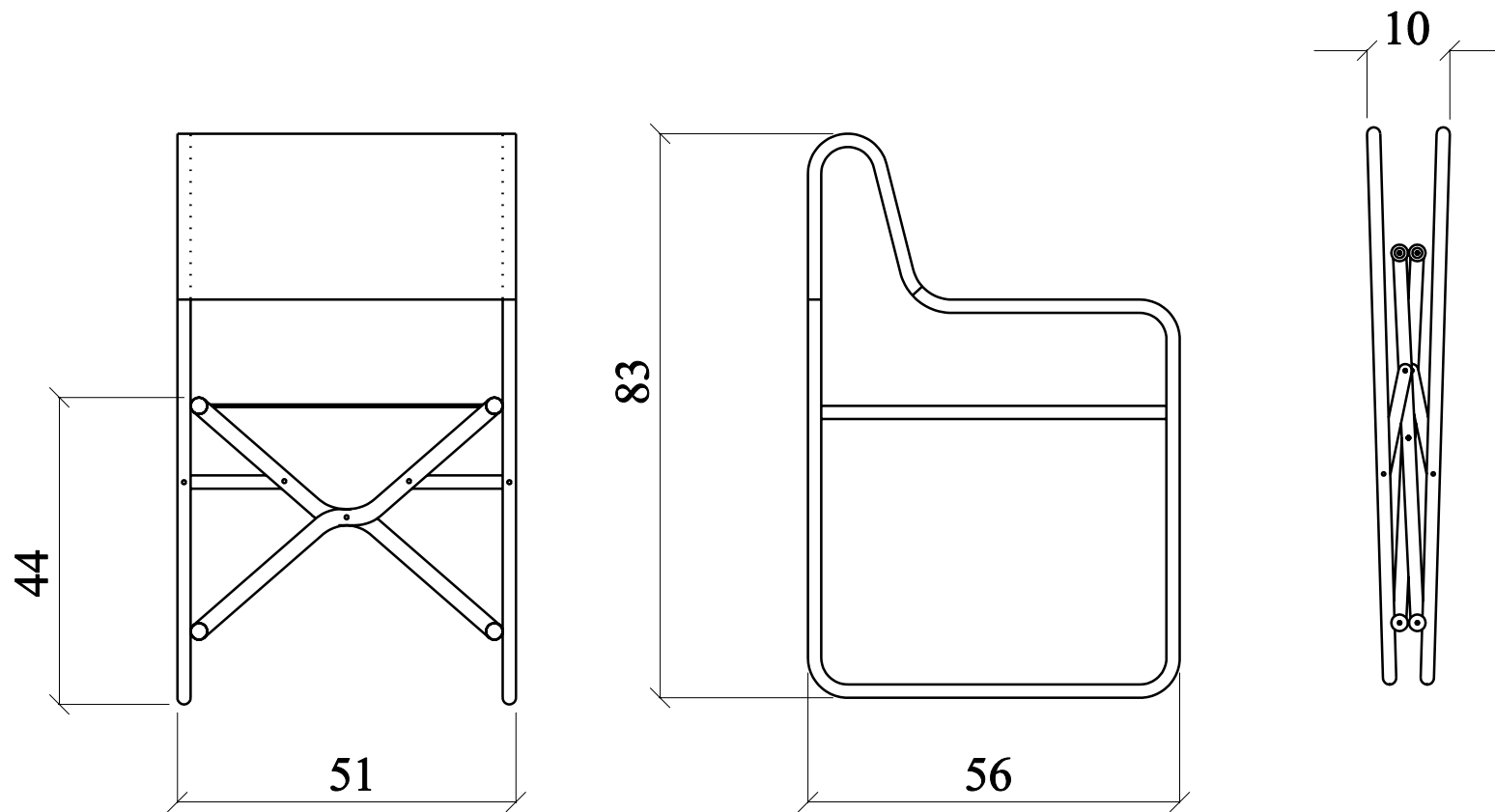
POLTRONCINA S/P/4 S/P/4 FOLDING ARMCHAIR
