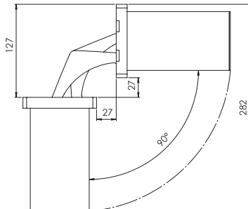
RECESSED HINGE B15, 90°
