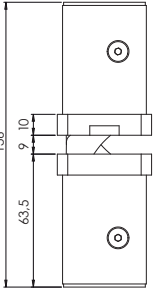
RECESSED HINGE B8, 0°
