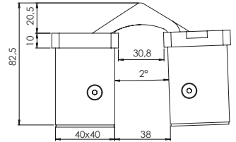
RECESSED HINGE B10, 178° (MAXIMUM OPENING)
