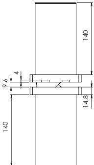
RECESSED HINGE B15, 0°
